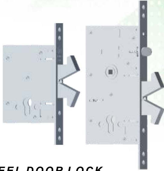
MONOBLOCK HOOKED STEEL DOOR LOCK
